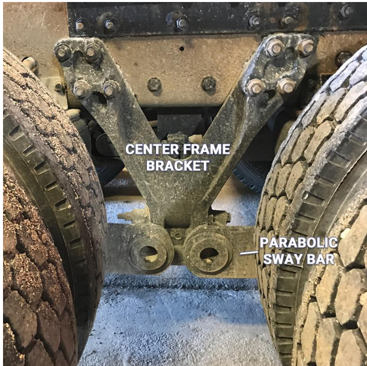
KENWORTH AIRGLIDE 200/400
