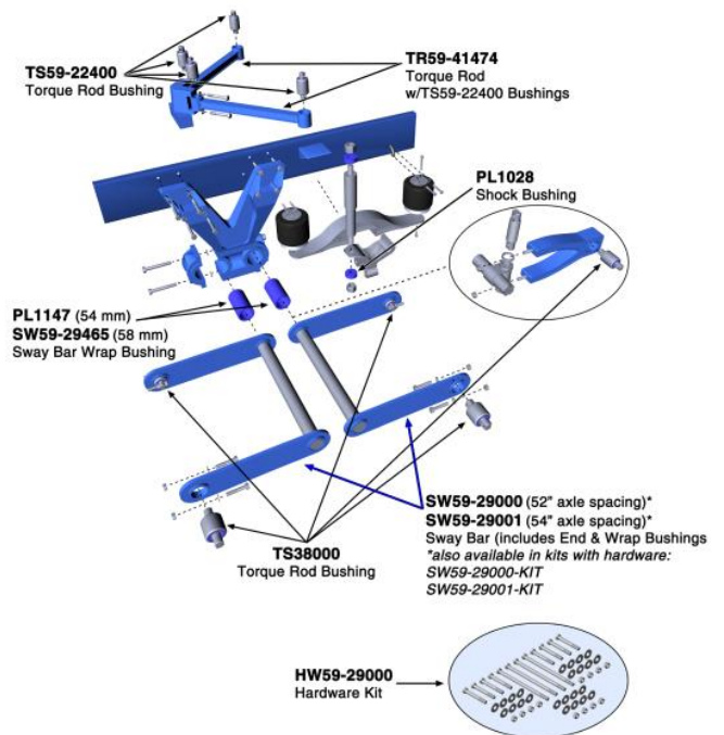
KENWORTH AIRGLIDE 200/400
