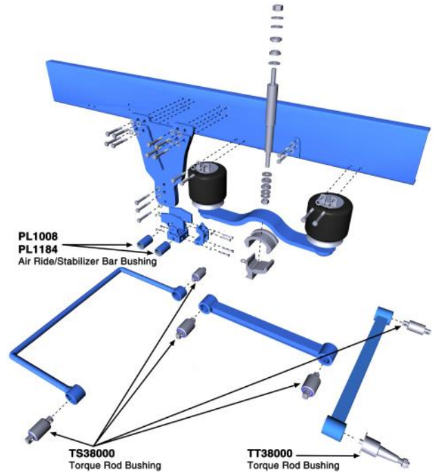
KENWORTH AIRGLIDE 100
